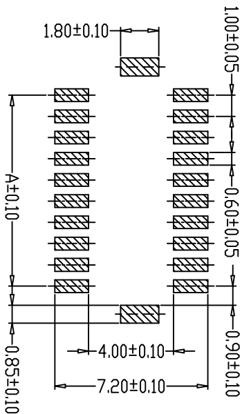
PCB LAYOUT
